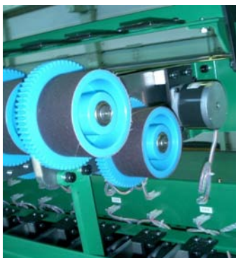
YARN FEED ROLL 4" DIAMETER
