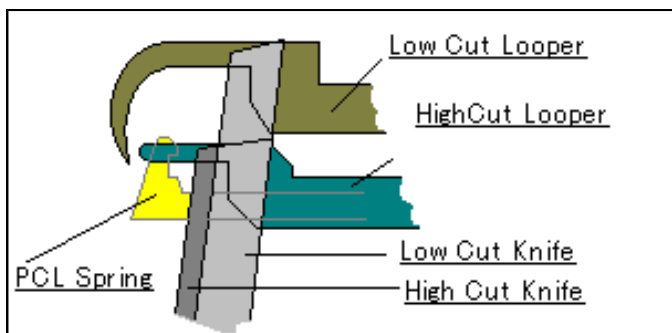
HIGH-CUT & LOW-CUT SYSTEM
