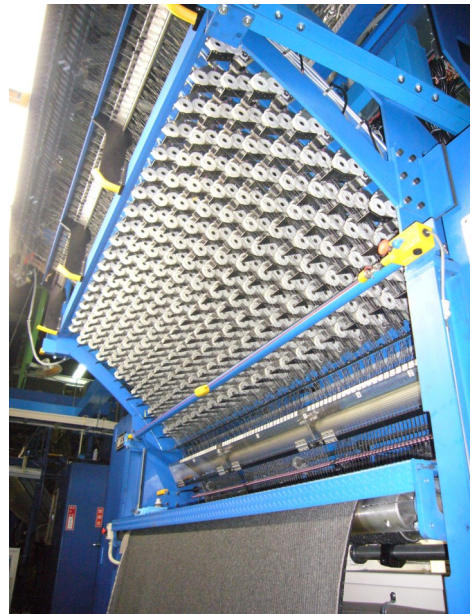
TUFTING MACHINE WITH “SHOGUN” SYSTEM
