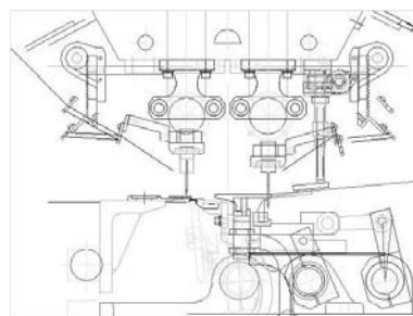
1/12" GG. TUFTING MACHINE
