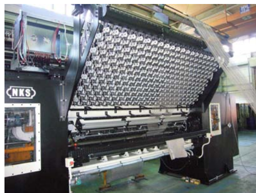
1/12" GG. TUFTING MACHINE
